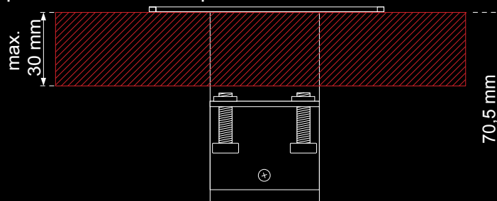
Assembly to table/desk top with thickness of up to 30 mm.
