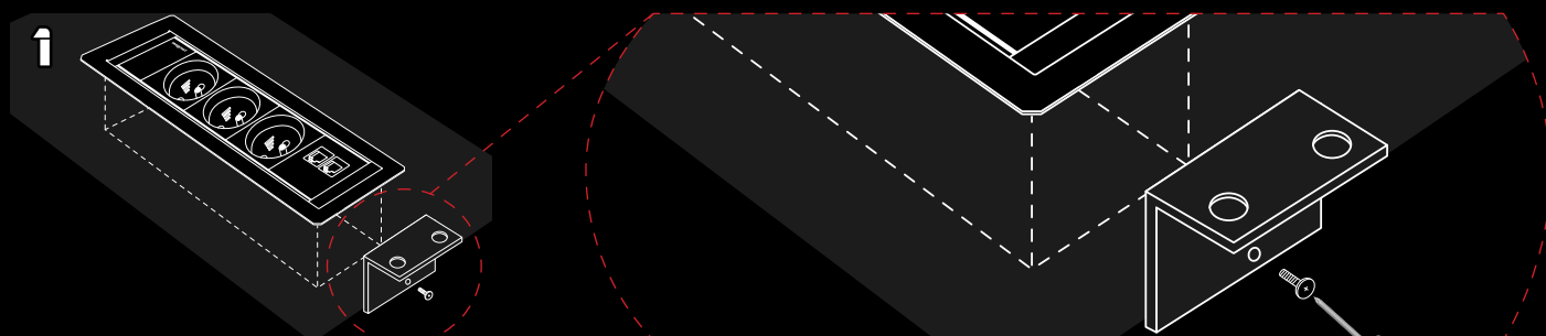
Insert Magnat-Frame into mounting hole and assembly of mounting brackets.
